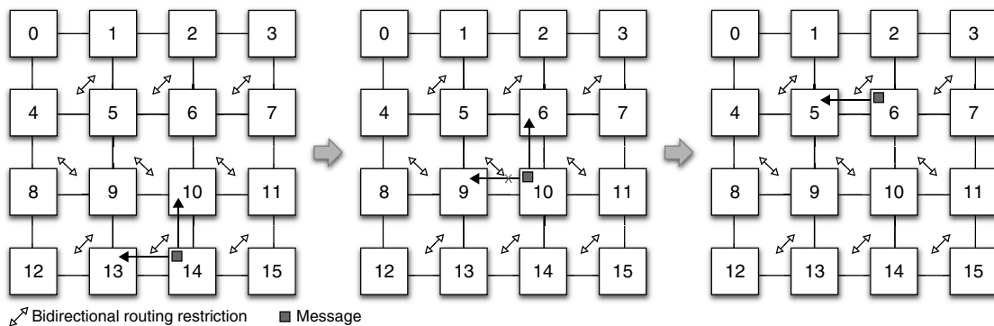
Figure F.25 Example of routing a message from Router 14 to Router 5 using LBDP at each router.
