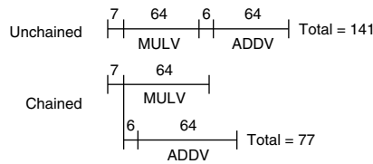
Figure G.8 Timings for a sequence of dependent vector operations ADDV and MULV, both unchained and chained. The 6- and 7-clock-cycle delays are the latency of the adder and multiplier.
