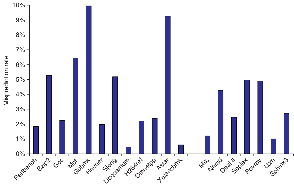
Figure 3.5 The misprediction rate for 19 of the SPECCPU2006 benchmarks versus the number of successfully retired branches is slightly higher on average for the integer benchmarks than for the FP (4% versus 3%). More importantly, it is much higher for a few benchmarks.
