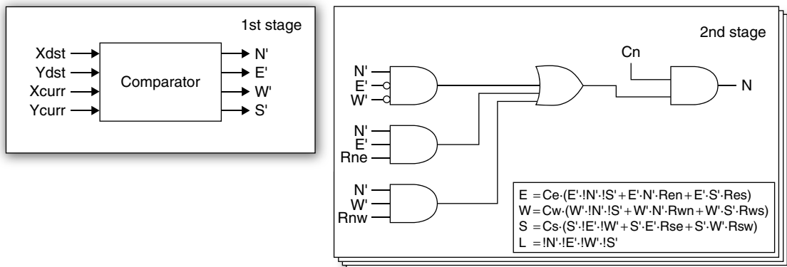
Figure F.24 LBDP logic at each input port of the router.
