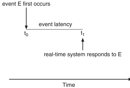
Figure 6.12 Event latency.
