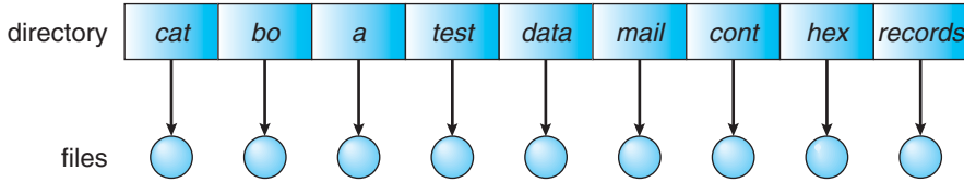
Figure 11.9 Single-level directory.
