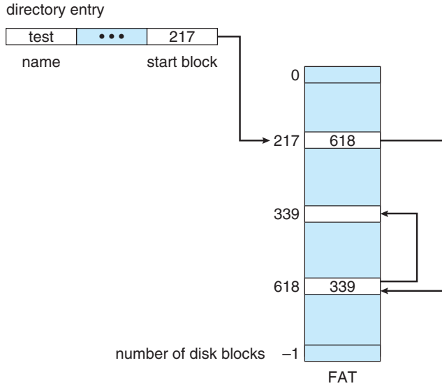
Figure 12.7 File-allocation table.
