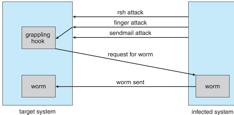
Figure 15.6 The Morris Internet worm.
