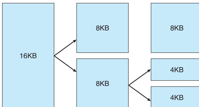
Figure 18.4 Splitting of memory in the buddy system.
