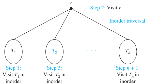
FIGURE 5 Inorder traversal.
