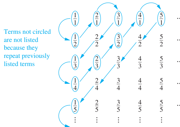
FIGURE 3 The positive rational numbers are countable.
