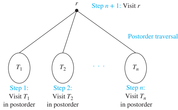
FIGURE 7 Postorder traversal.
