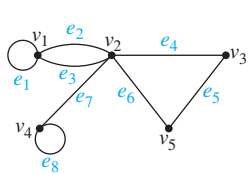
FIGURE 7 A pseudograph.
