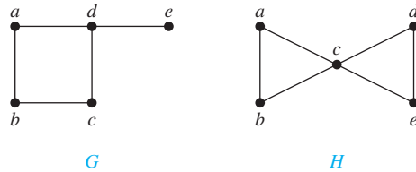
FIGURE 11 Two graphs that do not have a Hamiltonian circuit.
