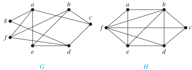
FIGURE 8 The undirected graphs G and H .
