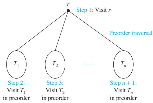
FIGURE 2 Preorder traversal.
