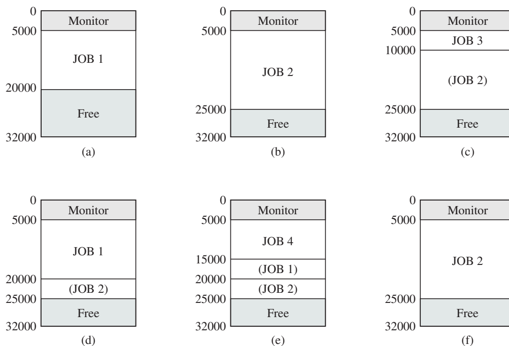
Figure 2.7 CTSS Operation
