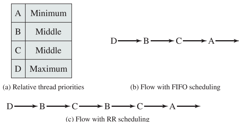
Figure 10.10 Example of Linux Real-Time Scheduling
