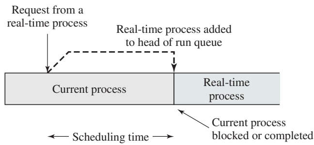
(b) Priority-driven nonpreemptive scheduler
