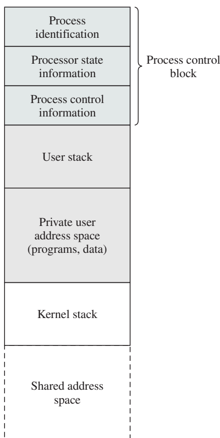
Figure 3.16 Process Image: Operating System Executes within User Space
