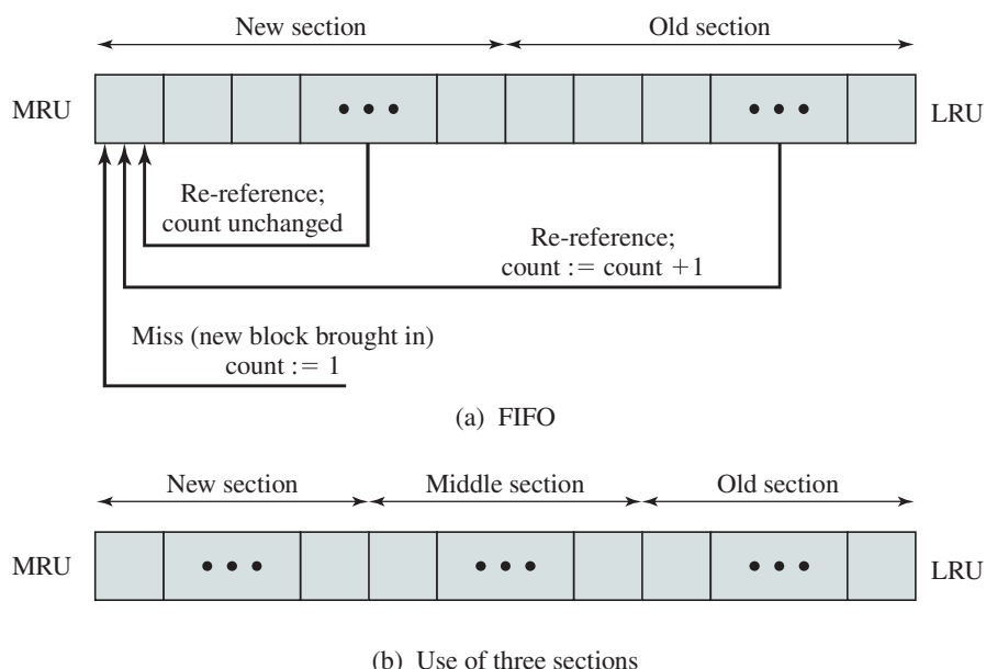
Figure 11.9 Frequency-Based Replacement
