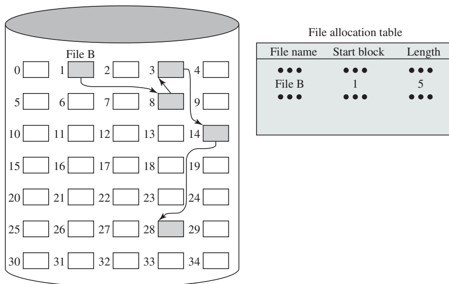
Figure 12.11 Chained Allocation
