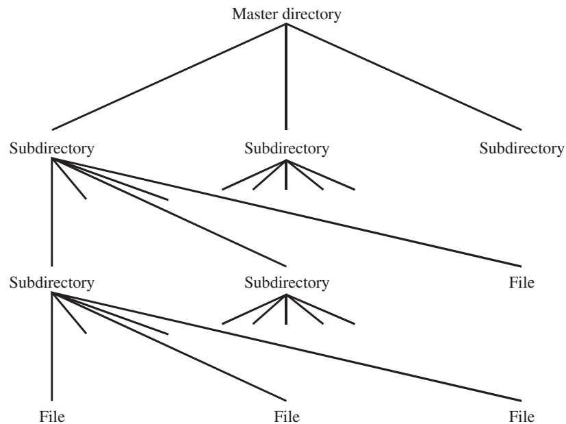
Figure 12.6 Tree-Structured Directory
