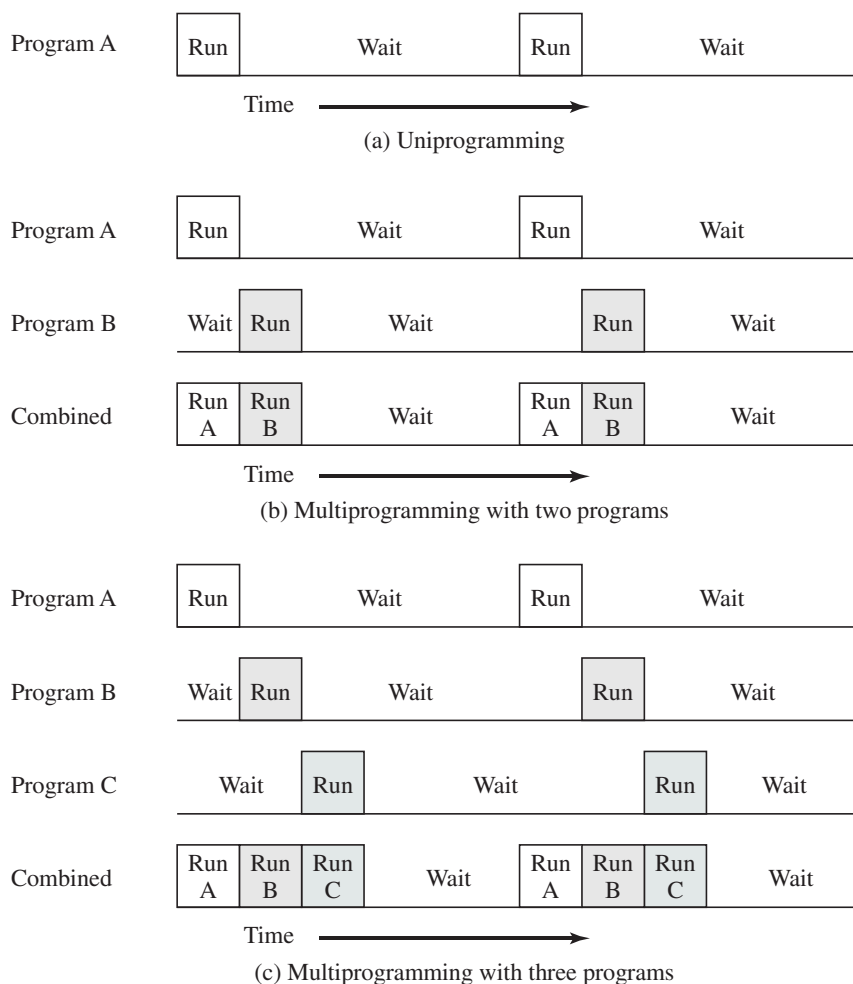
Figure 2.5 Multiprogramming Example
