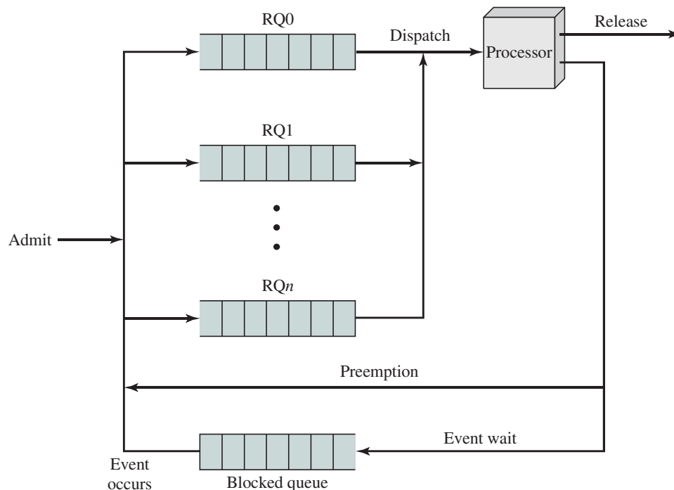
Figure 9.4 Priority Queuing
