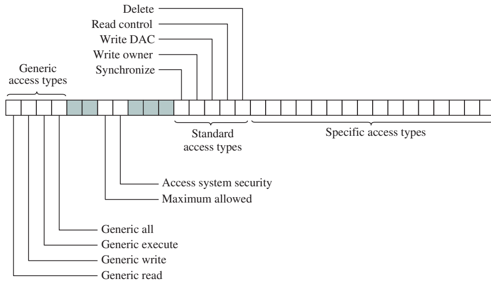
Figure 15.12 Access Mask
