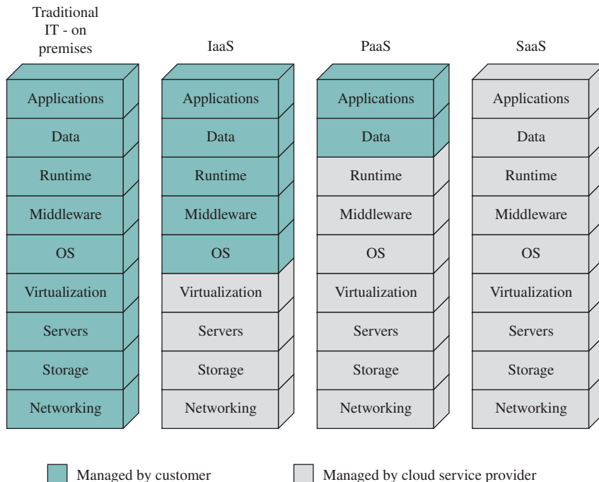
Figure 16.2 Separation of Responsibilities in Cloud Operation www.youseficlass.ir
