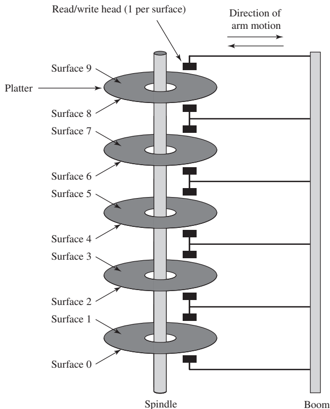
Figure J.3 Components of a Disk Drive www.youseficlass.ir
