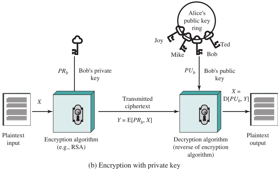
Figure K.2 Public-Key Cryptography
