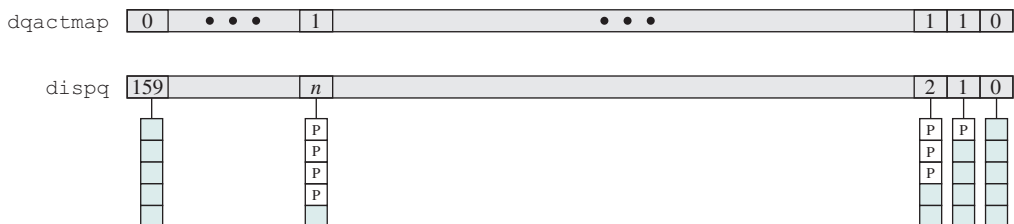
Figure 10.13 SVR4 Priority Classes
