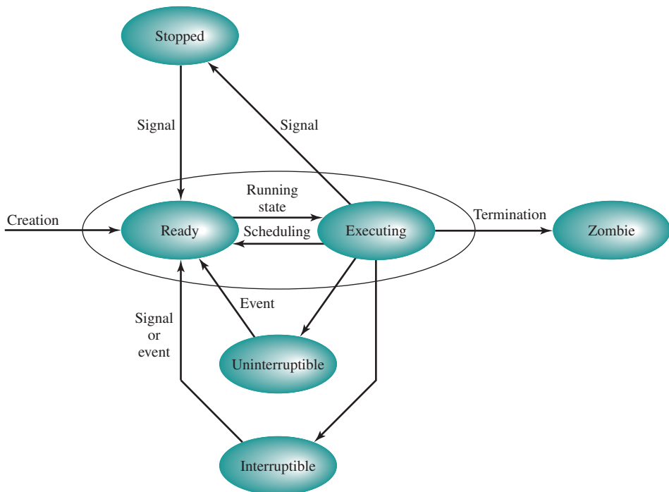
Figure 4.15 Linux Process/Thread Model www.youseficlass.ir
