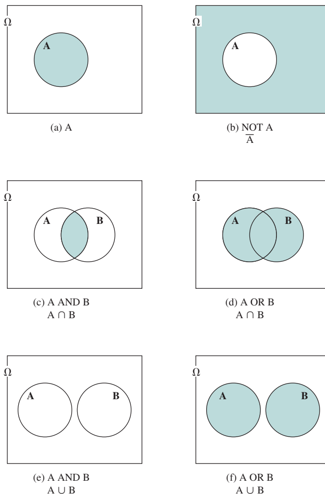
Figure 20.1 Venn Diagrams
